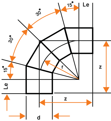
Elbow 90°
